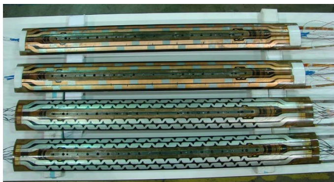
Fig. 6. Coil assembled in the first MQXF short models: from bottom to top, coil 03 and 05 fabricated by LARP) and coil 103 and 104 (fabricated by CERN).
