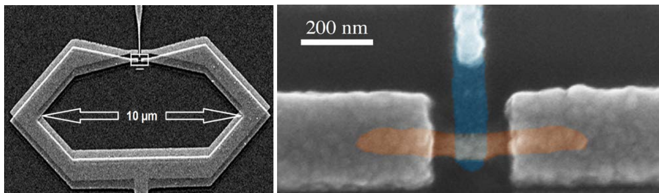
Fig. 1. (left) Scanning electron micrograph of the SQUIPT loop geometry with the weak link inserted in the top of the ring. The ring itself is made out of three layers in the EBL fabrication process involving three angle shadow evaporation through a suspended mask: at first, a thin layer of aluminum (15 nm) is deposited with an oxide tunnel barrier on top, then the copper film (20 nm) and finally a thick (100 nm) aluminum layer. The box around this weak link marks the extent of the area depicted on the right (colored SEM image): a small normal conducting copper strip interrupts the thick superconductor. In addition, a superconducting (blue) contact is attached via a tunnel barrier to the middle of the weak link.
