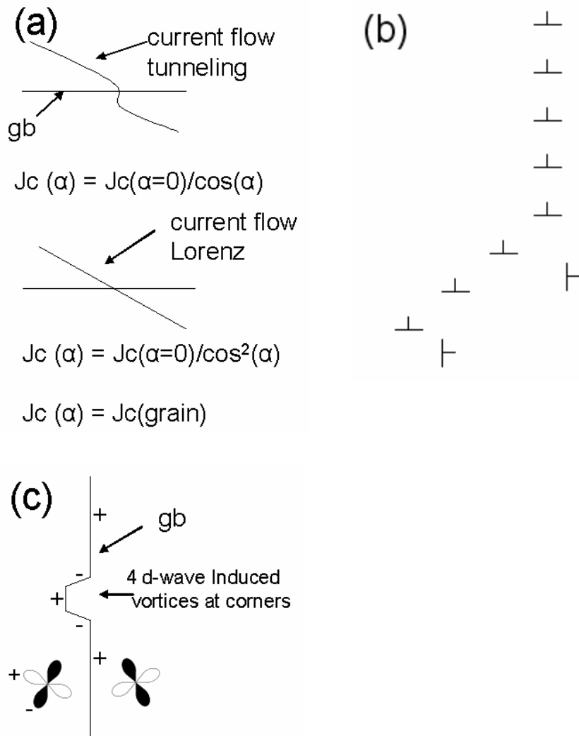
Figure 1. Schematic drawings of three experiments proposed in the text. (a) A sketch indicating current flow at an angle \alpha from the normal to the grain boundary plane marked gb, indicated as a horizontal line, see Feldmann et al [10]. (b) Edge dislocation array in a symmetrical grain boundary plane is the vertical array. Additional dislocations as the grain boundary plane meanders to the left. (c) A vertical grain boundary plane in which appreciable Josephson is present is tilted twice by a second phase as the grain boundary meanders and is bound around it. For an example see the photomicrograph in Feldmann et al [10]. Additional d-wave vortices are formed and pinned spatially.
