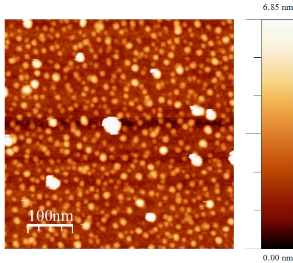
Figure 1. AFM image of Ag nanodots on STO substrate deposited at temperature of 450 °C in vacuum with 15 laser pulses.
