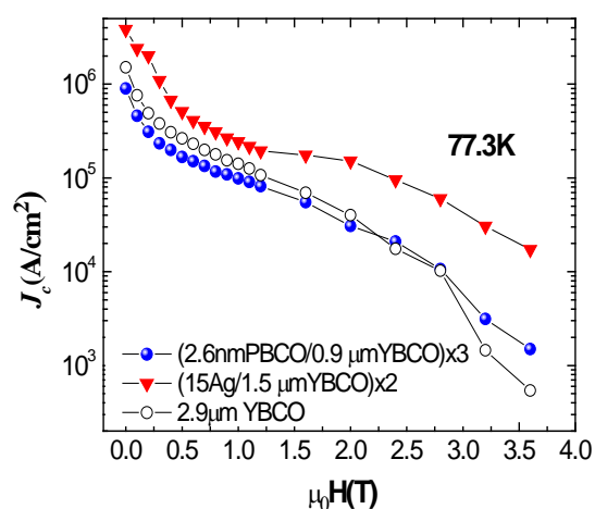
Figure 3. J_c(H) dependence in Ag/YBCO quasi-multilayer with the total thickness of 3 \mu\text{m} , PBCO/YBCO quasi-multilayer of the thickness of 2.7 \mu\text{m} and reference pure 2.9- \mu\text{m} YBCO film. The legend indicating samples is shown in the plot.
