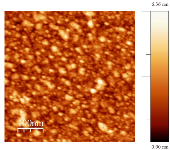
Figure 2. AFM image of PBCO nanodots on STO substrate deposited at temperature of 450 °C in vacuum with 15 laser pulses.
