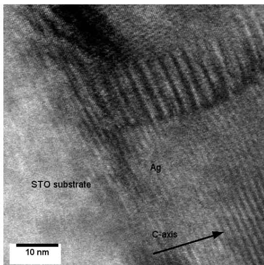
Figure 9. TEM image of Ag/YBCO quasi-multilayer taken at the interface with STO substrate.
