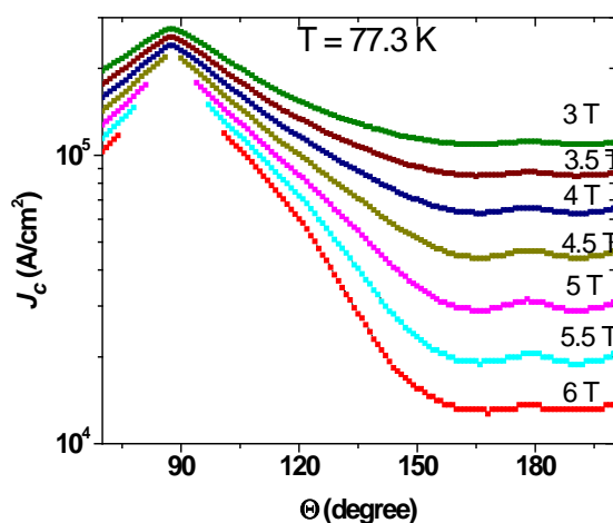
Figure 5. Angular dependence of critical current density in Ag/YBCO quasi-multilayer at different magnetic fields from 3 to 6 T at temperature of 77.3 K
