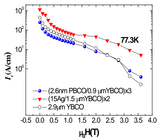
Figure 4. Total critical current per centimetre of width as function of magnetic field I_c(H) for the same samples as in Fig 3.
