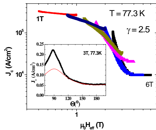
Figure 8. Best scaling of J_c(\theta, H) at 77.3K assuming \gamma = 2.5 in PBCO/YBCO quasi-multilayer. Inset: total value of J_c(\theta) at 77.3 K and 3 T (black points) and the uncorrelated defects contribution (red line).
