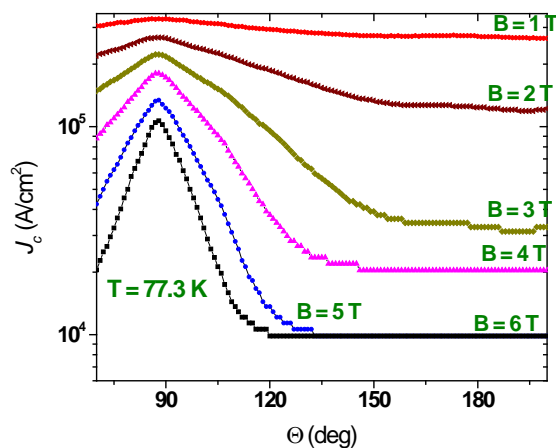
Figure 7. Angular dependence of critical current density in PBCO/YBCO quasi-multilayer at different magnetic fields from 1 to 6 T at temperature of 77.3 K
