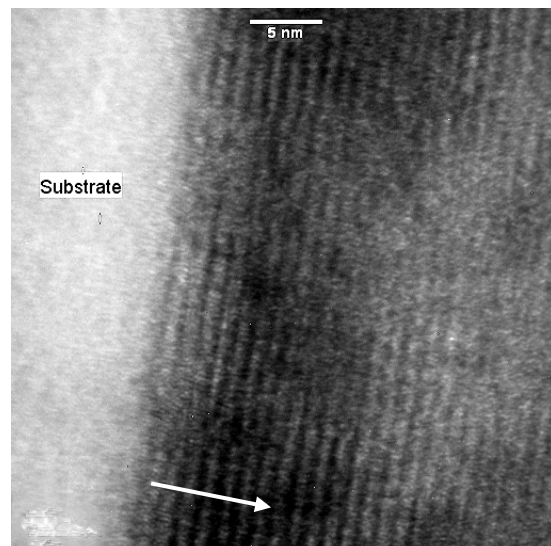
Figure 10. TEM image of PBCO/YBCO quasi-multilayer taken at the interface with STO.
