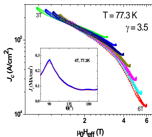
Figure 6. Best scaling of J_c(\theta, H) at 77.3 K assuming \gamma = 3.5 in Ag/YBCO multilayer. Inset: total value of J_c(\theta) at 77.3 K and 4 T (blue points) and the uncorrelated defects contribution (red line).
