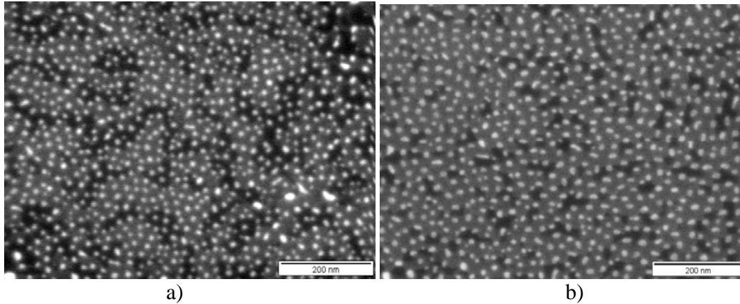
FIGURE 6. SEM photomicrograph showing uniform BSO distribution in YBCO on a) 260 nm sample and a b) 2.8 μm sample
