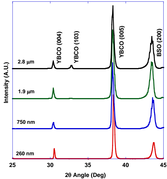
FIGURE 4. \theta - 2\theta x-ray scans of YBCO + 20 mol% BSO of varying thickness.
