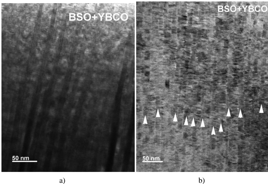
FIGURE 7. Cross sectional TEM image showing through-thickness, uniform BSO nanocolumns in a) 780nm film and a b) 2.8 μm film
