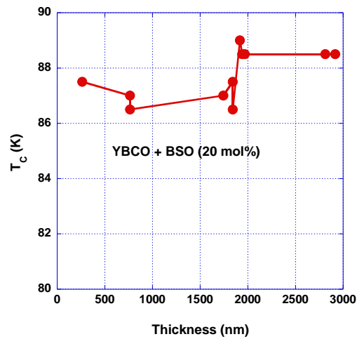
FIGURE 1. T_C in YBCO + 20 mol% BSO films with varying thickness.
