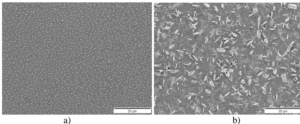
FIGURE 5. SEM photomicrograph showing surface microstructure of a) 260 nm sample and a b) 2.8 \mu\text{m} sample
