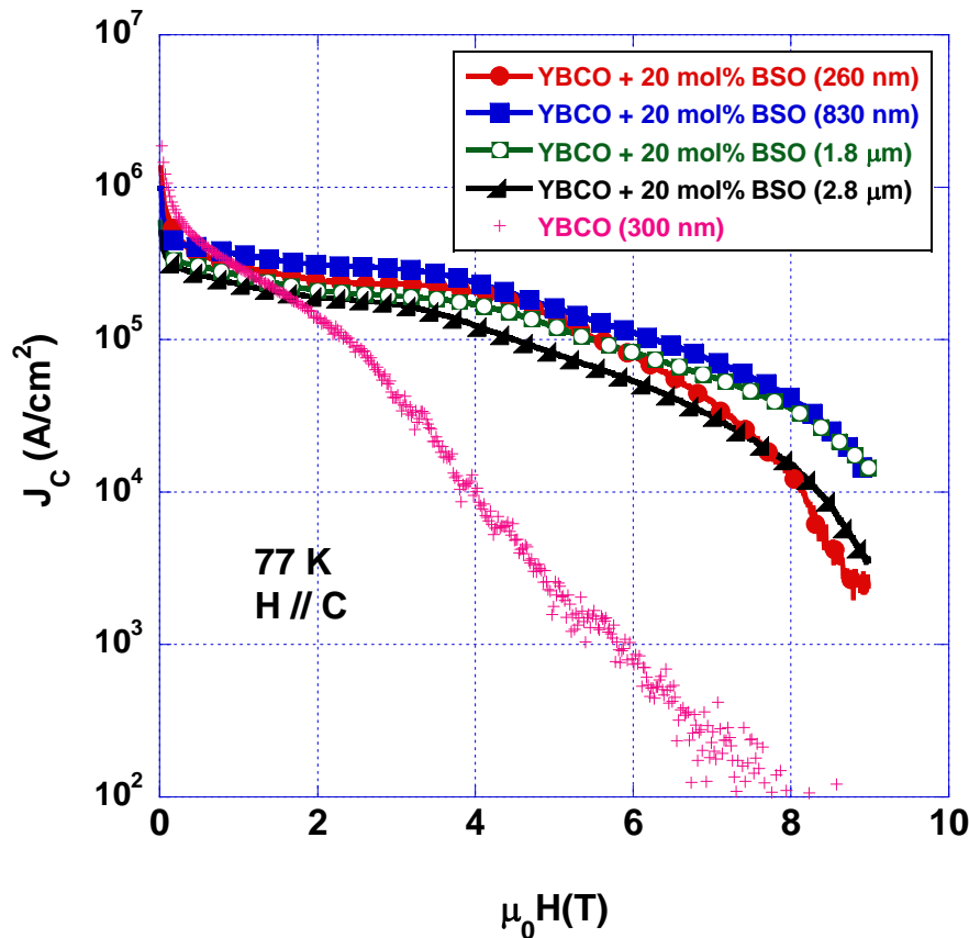
FIGURE 3. VSM J_C data for selected YBCO + 20 mol% BSO film thicknesses compared with 300 nm YBCO at 77 K and H // c .
