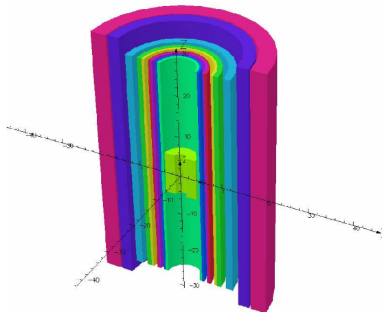
Fig. 6. Schematic of the integrated LTS-HTS 22.5 Tesla magnet system. The HTS insert is the innermost green coil, the two outermost coils are NbTi and the remainder are Nb 3 Sn coils.
