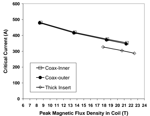
Fig. 4. The critical current (0.1 μV/cm criterion) at 4.2 K of the two coaxial inserts coils and the quench current of the thick insert plotted against the peak magnetic flux density generated in the coil. The coaxial coils are powered separately. The background field generated by the LTS outer was 6.7 T, 12 T, 17 T and 20 T for the four data points for each coaxial coil, and 15 T, 18 T and 20 T for the three data points of the thick insert.
