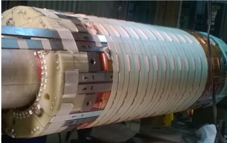
Inner Coil
