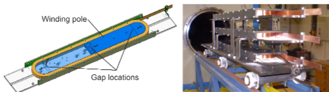
Fig. 2. Design of the fixture for the dilatation test (left) and insertion of three fixtures in the reaction oven (right).
