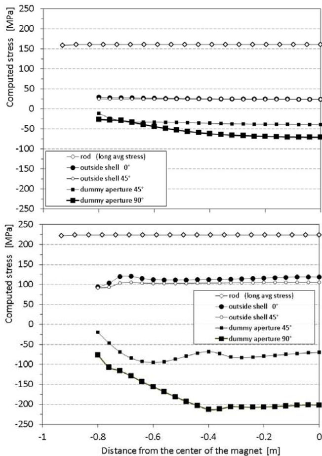
Fig. 9. Computed stress in shell outer shell (azimuthal), inner surface of dummy coil aperture (azimuthal) and axial rods (longitudinal) vs. z position.
