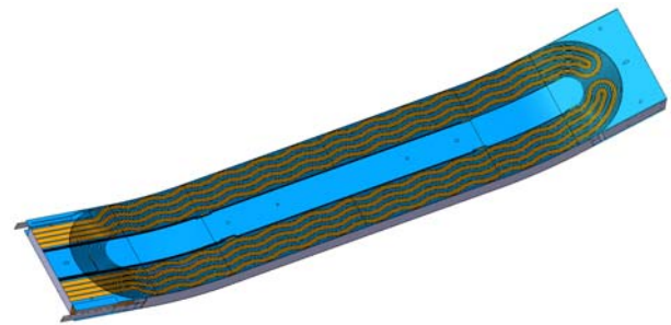
Fig. 10. Quench heater trace design.
