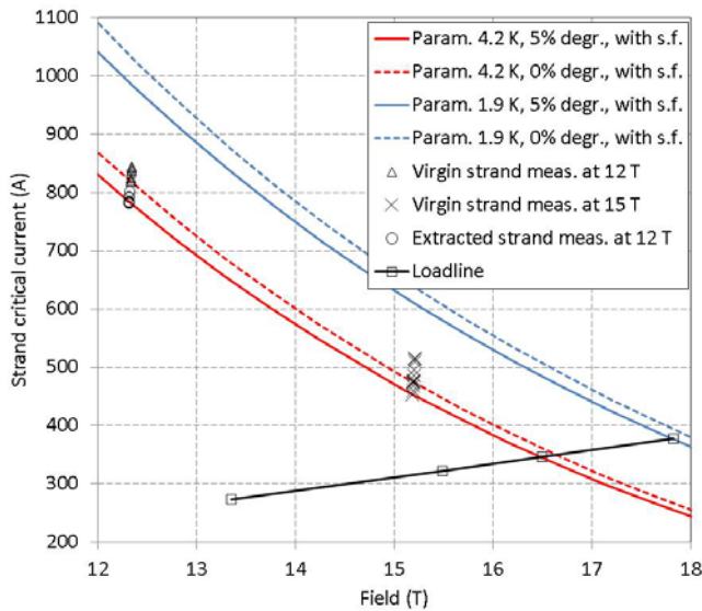
Fig. 1. Strand critical current (A) vs. total magnetic field (T) measurements and parameterization curves of virgin strands (no degradation) and extracted strands (5% cabling degradation), together with magnet load-line.
