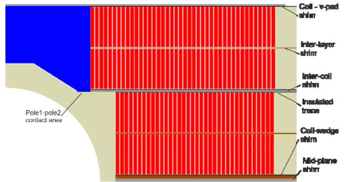
Fig. 3. Coil cross-section and insulation scheme.
