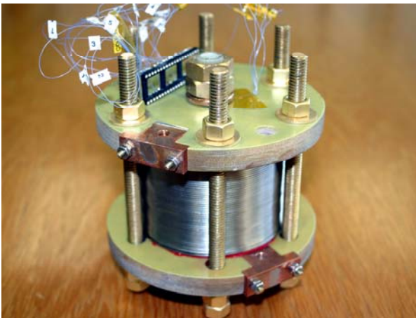
Fig. 7. Photo of high field insert coil fabricated at SuperPower with standard SCS4050 2G HTS wire. At 4.2 K, the coil generated a self field of 9.8 T and a center field of 26.8 T when placed in a 19 T axial background field. Flange diameter is 127 mm.
