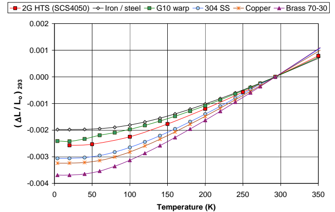
Fig. 5. Thermal expansion of standard production (SCS4050) SuperPower 2G HTS wire compared with other common magnet construction materials.
