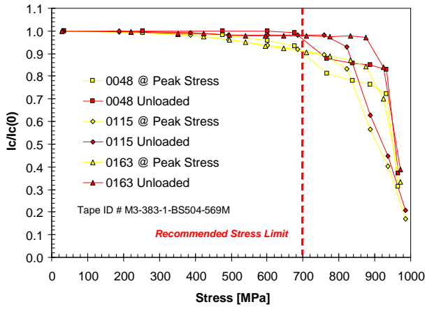
Fig. 2. Plot of normalized critical current ( I_c / I_c(0) ) vs. applied axial stress on a 4 mm wide, standard production SuperPower® 2G HTS wire. A stress limit of 700 MPa is recommended.
