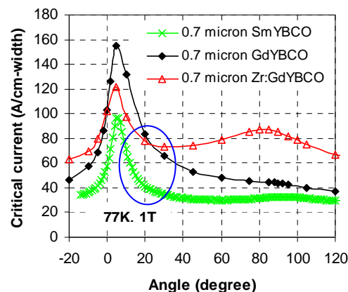
Fig. 1. Critical current as a function of angle between magnetic field and film surface at 77 K, 1 T for 12 mm wide samples with same film thickness but different film compositions. The green line is representative of current standard production tape with Sm doping. The black and red lines are representative of improved conductors with Gd and/or Zr substitution into the REBCO structure. The critical region for coil performance is given in blue.
