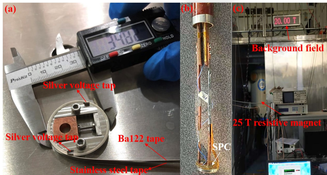
Figure 1. The outer view of Ba122 single pancake coil with 30 mm inner diameter (a), the sintered Ba122 SPC (b) and the 25 T resistive magnet (c) [8].
