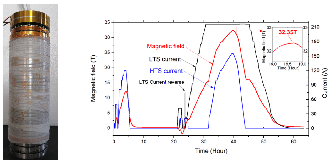
Fig.1. The REBCO insert (left) and the excitation process at 4.2 K (right). During the excitation process, the current direction of the LTS magnet was changed one time as shown in the figure, since the direction of the magnetic field generated by the LTS magnet was against the direction of the magnetic field generated by the HTS insert.
